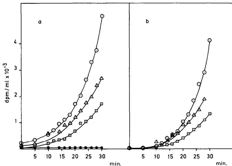
Fig. 1. Specific radioactivity of total protein in the supernatant of the cell suspension (dpm/ml) after addition of L-[1- ^{14} C]leucine, in dependence of the incubation time (min). ( \square — \square ) 2 \mu Ci/ml; ( \Delta — \Delta ) 5 \mu Ci/ml; ( \circ — \circ ) 10 \mu Ci/ml; ( \bullet — \bullet ) 2 \mu Ci/ml plus 0.4 mg/ml puromycin. a: Measured curves. b: calculated curves, after subtraction of the linear component from the measured curves.
